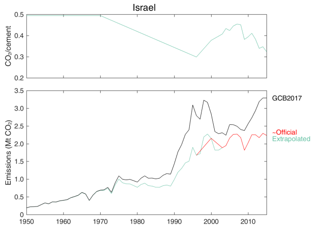
Figure C21. Revised cement emissions in Israel.
